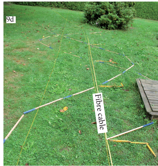
Figure 9d: The two contours of a double helix around a fibre-optical cable are indicated schematically with wooden sticks. The yellow scales mark the positions of measurement.
