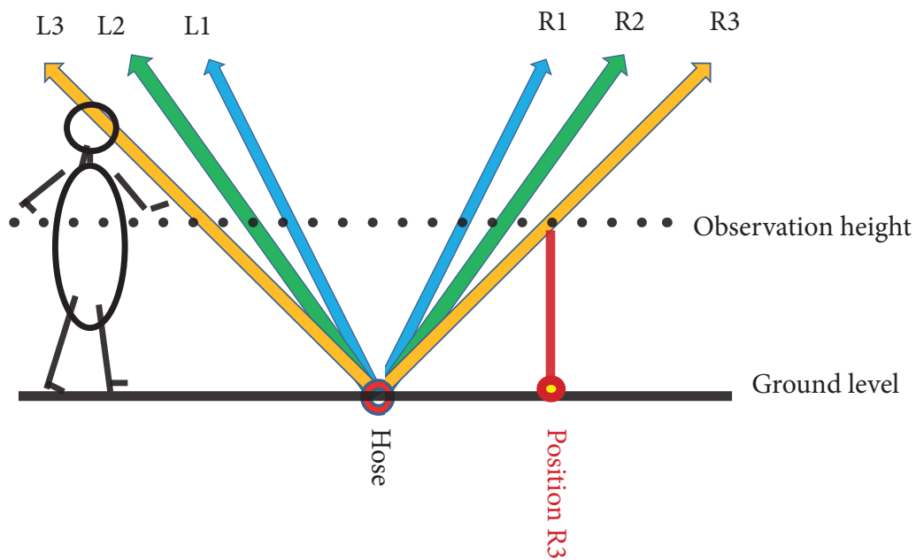
Figure 9a: View in the axial direction of the hose: The zones are observed at a height of about 1 m, and their positions are projected downward to ground level.
