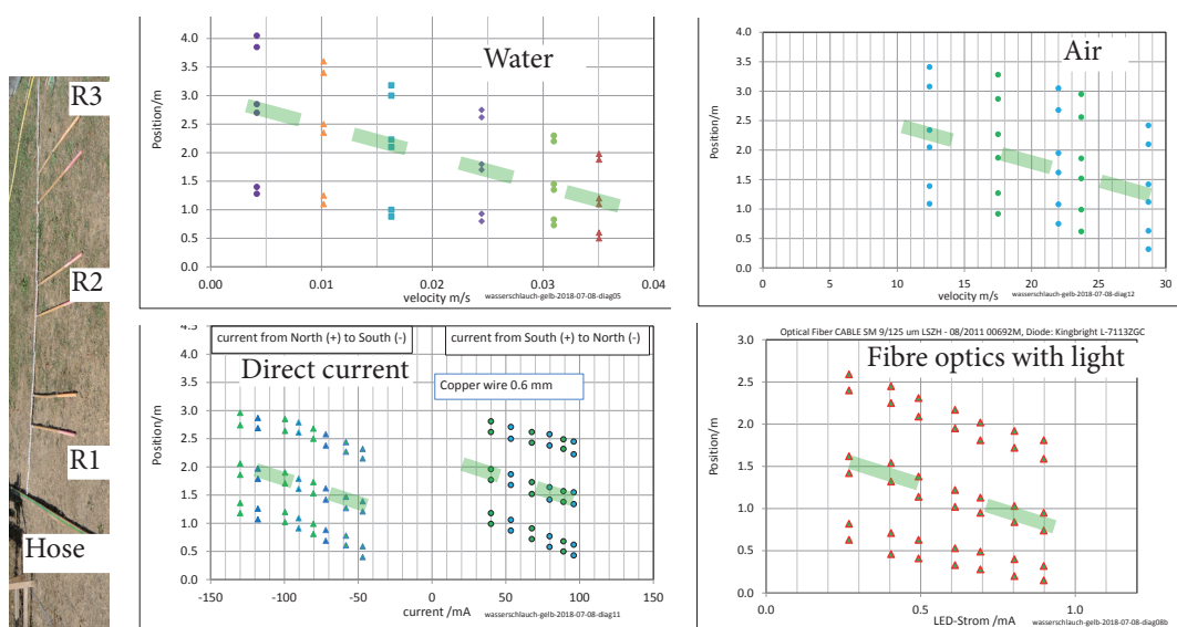
Figure 21: Comparison of properties for the zones generated with water, air, direct current, and light (see figures 9b, 17e, 18d and 19d)
