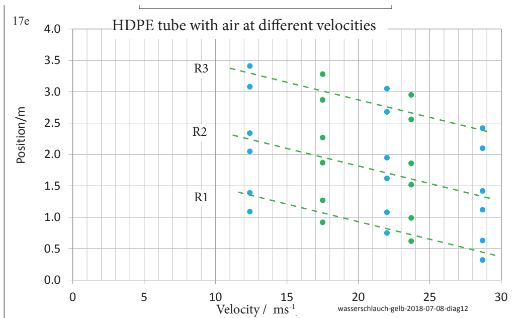
17e: Positions of zones R1, R2, and R3 with air flowing through a plastic (HDPE) pipe at different velocities
