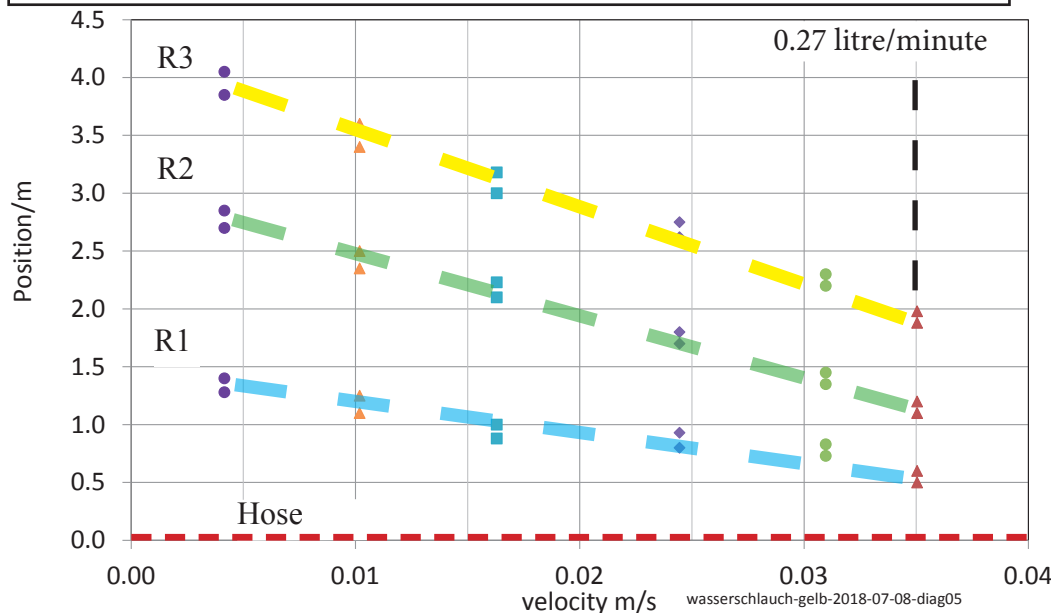
Figure 9b: The positions of the zones R1 to R3, are shown for various flow velocities, each at the left- and right-hand edges. Water hose yellow
