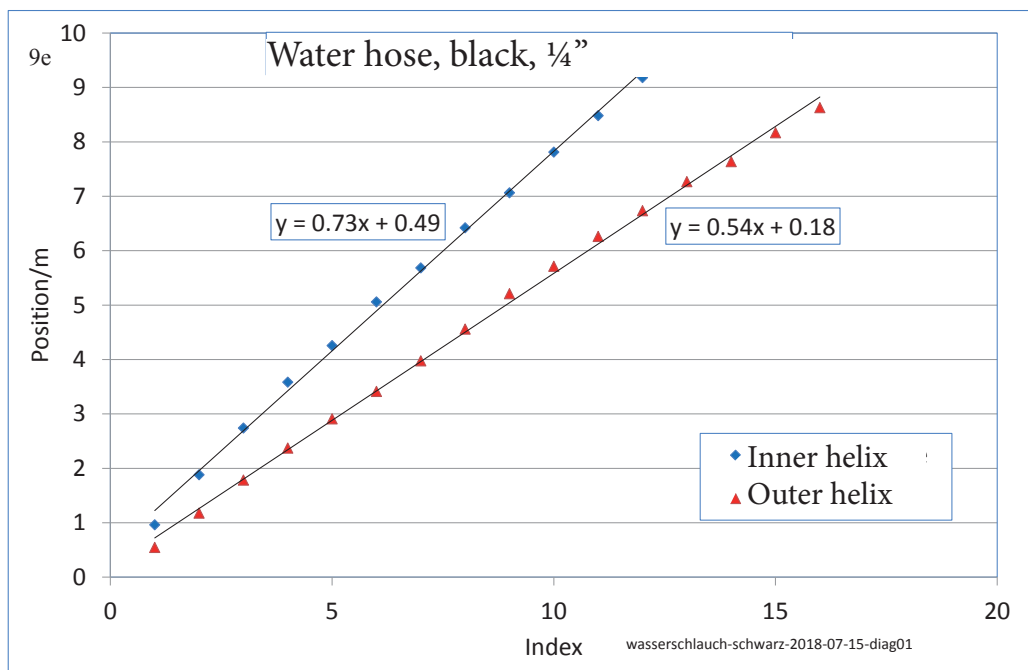
Figure 9e: Two double helices which wind around a \frac{1}{4} " hose extend in the longitudinal direction: The positions of the maxima found for the inner as well as the outer helices are each plotted along a consecutive number. This representation provides a simple overview. If the distances are uniform, the sequence of points can be approximated quite well by a straight line. The slope of this line is then the average distance. In this case, the straight lines fit well and yield values of 0.54 m and 0.73 m.
