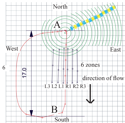
Figure 6: Arrangement of the elements (The grid is graduated in metres. The positions of the points have been determined with a tachymeter. The lines and circles are only schematic.)
