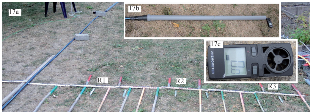
Figure 17: Hard plastic (PE) pipe with flowing air 17a: The inner and outer edges of zones R1, R2, and R3 have been correspondingly marked for different flow velocities. On the wooden sticks, the colour green indicates the highest velocity, and the colour orange indicates the lowest velocity. 17b: For determining the flow velocity, the end of the pipe is concluded with a section of 40 mm HT pipe. 17c: Anemometer
