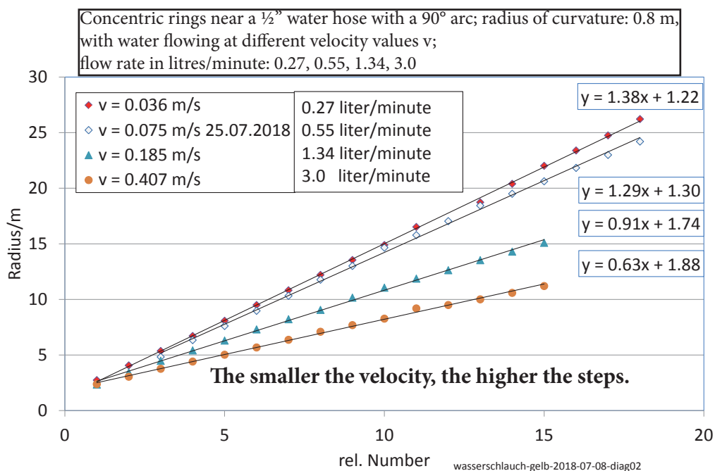
Figure 13: Measured radii of the ring-shaped structures for different flow rates of the water
