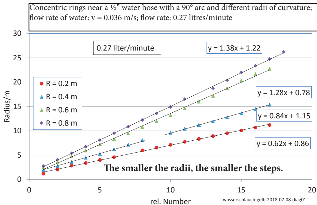
Figure 12: Measured radii of the ring-shaped structures for different radius of curvature of the arc (Refer to the comment from figure 9b for the type of representation.)
