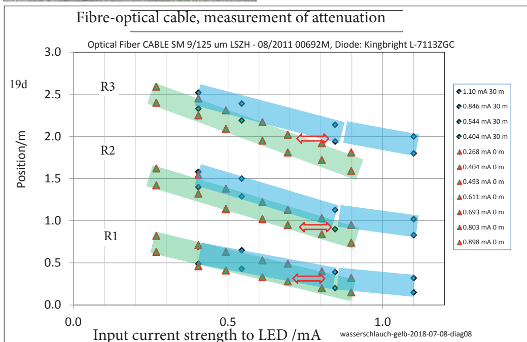
Figure 19: Zones associated with a fibre-optical cable, left and right edge, respectively
