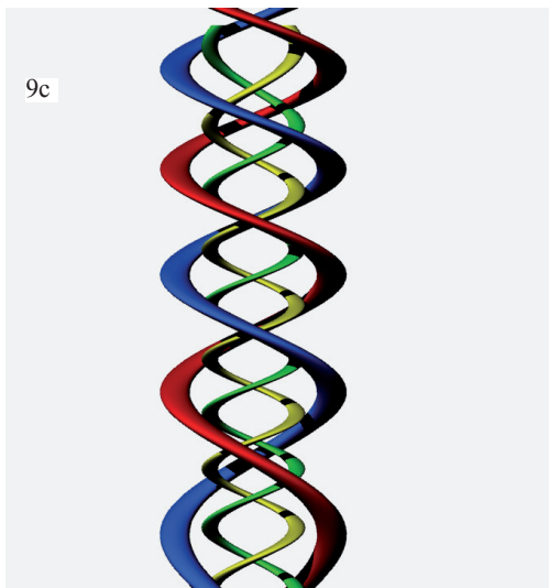
Figure 9c, schematic diagram: Two double helices are present around the hose. In comparison with the outer helices (blue and red), the inner helices (green and yellow) have a shorter lead, a smaller radius, and the opposite sense of rotation.
